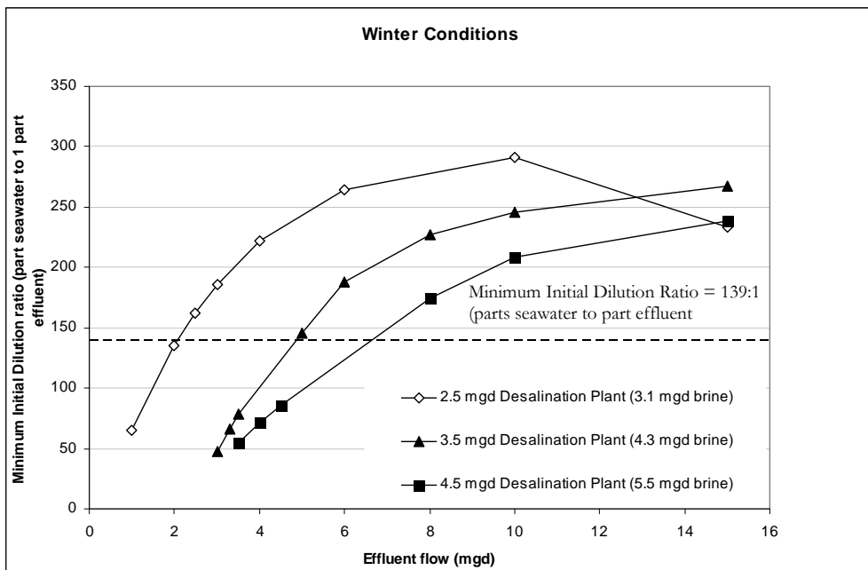
Figure 5-1(b). Dilution Factors under Three Desalination Alternatives as a Function of Increasing Wastewater Effluent Flow Rates during Winter Conditions
